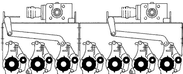
7 Scroll Shafts (3+4)
