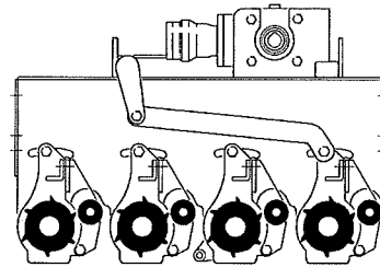
4 Scroll Shafts
