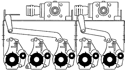
5 Scroll Shafts (3+2)
