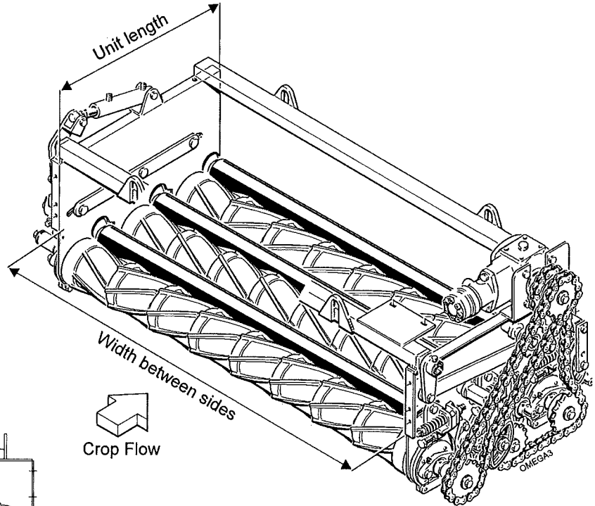
4 Scroll Shafts
