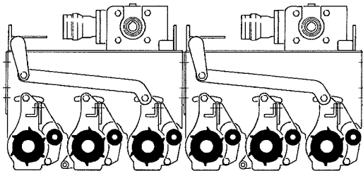
6 Scroll Shafts (3+3)
